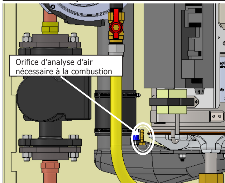
FIGURE 9-6 Combustion Analyzer Port - 299
