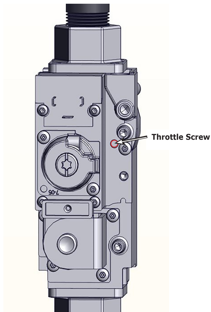
FIGURE 9-4 Gas Valve - Model 299 MBH
