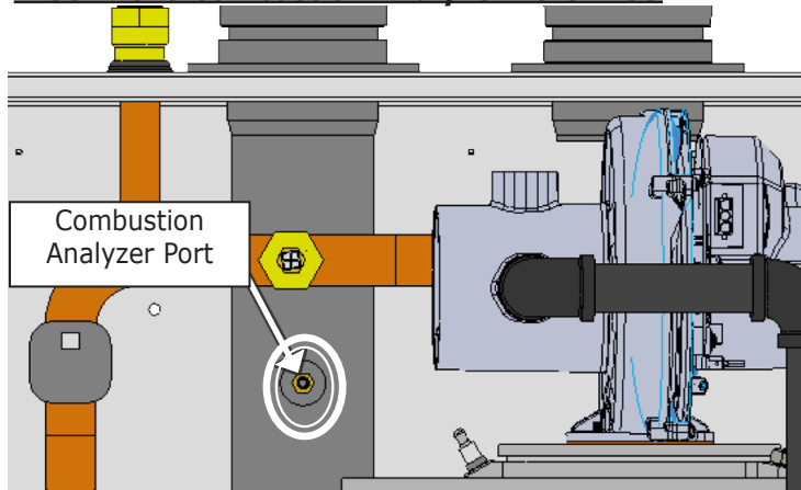
FIGURE 9-6 Combustion Analyzer Port - 299
