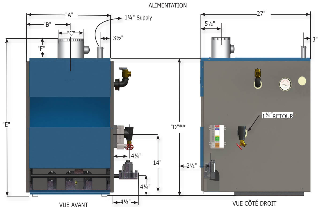
Figure 1 - Dimensions
