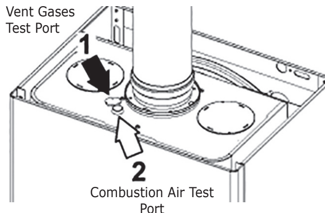
Figure 18 - Test Ports
