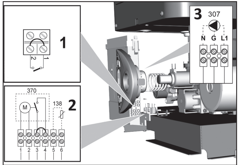
Figure 17 - Terminal Block
