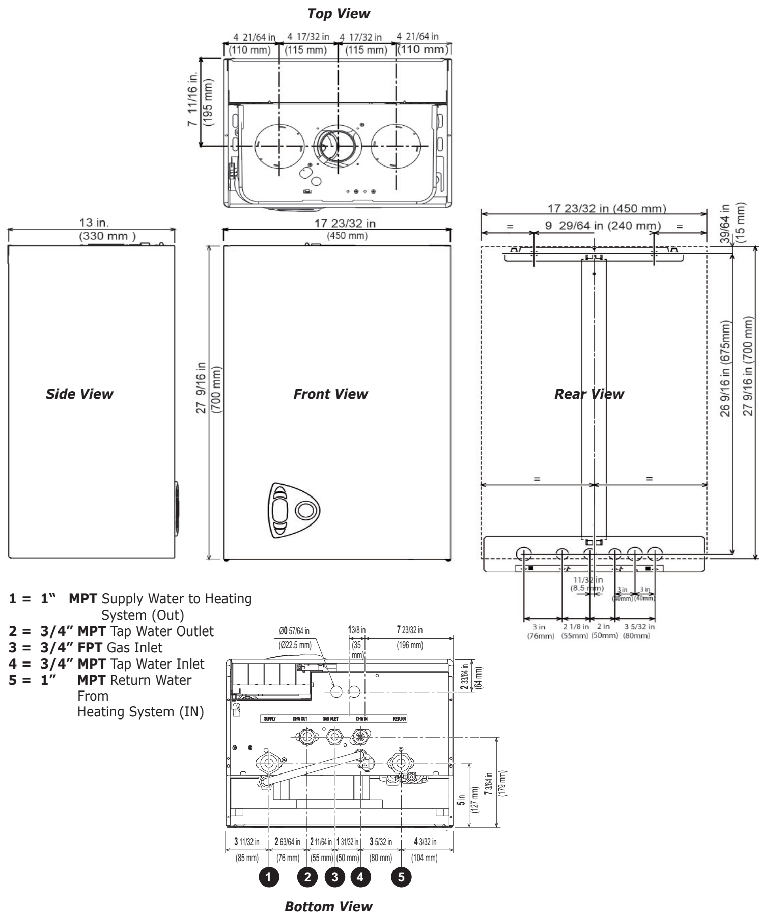
Figure 1 - Overall Dimensions
