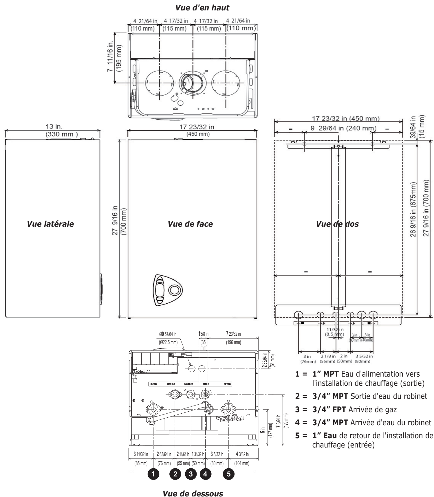
Figure 1 - Dimensions
