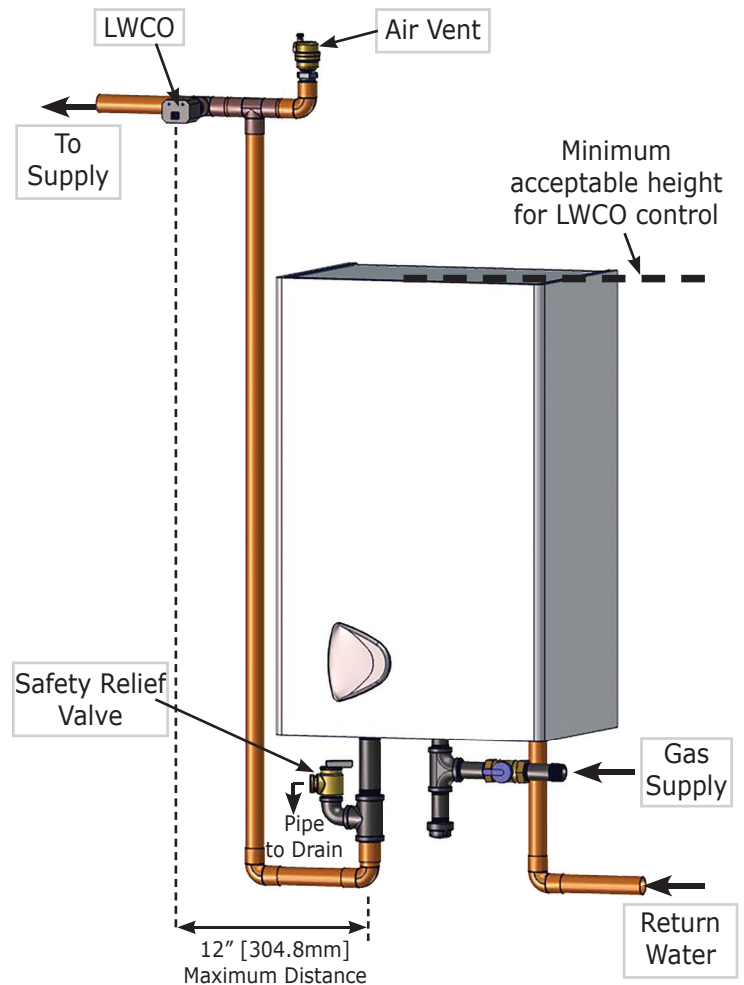
Figure 9 - LWCO Suggested Probe Location
