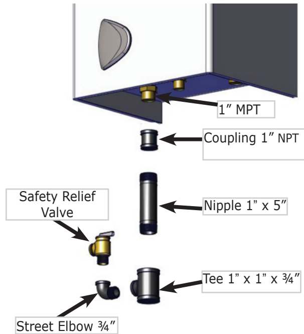
Figure 8 - Safety Relief Valve Discharge Piping
