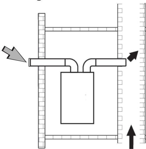
Figure 15 - Chimney Venting with Outside Air Single Wall
