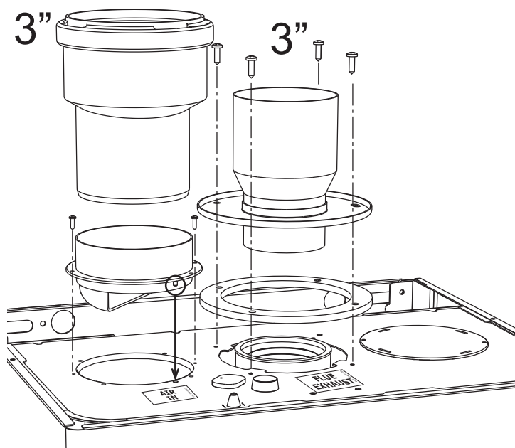
Figure 11 - Combustion Air Fitting
