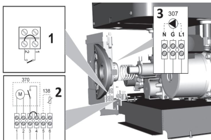
Figure 17 - Bornier
