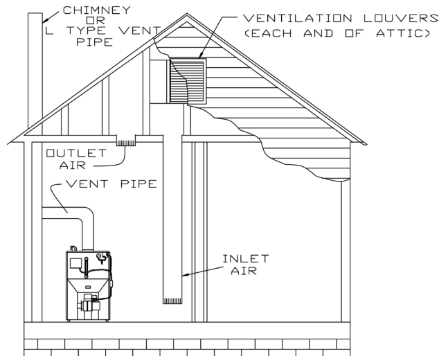
Figure 4 Vertical Ducts
