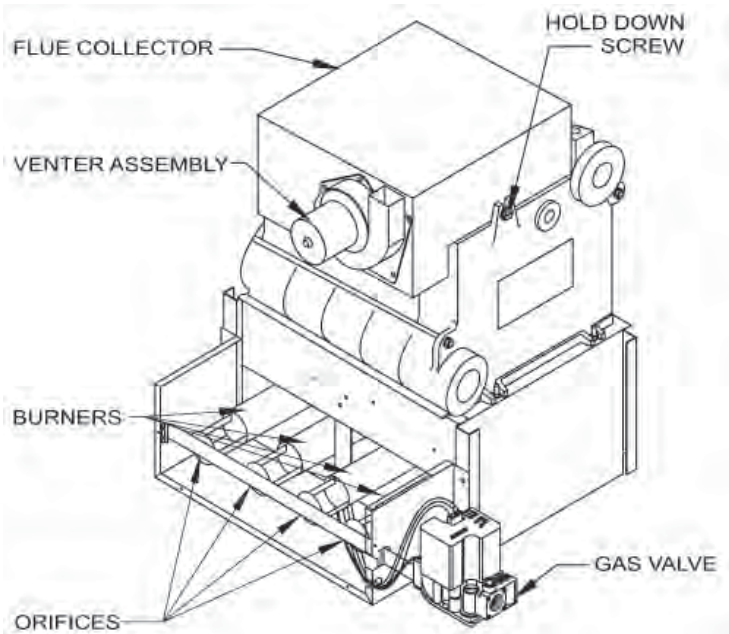
Figure 4 - Flue Collector
