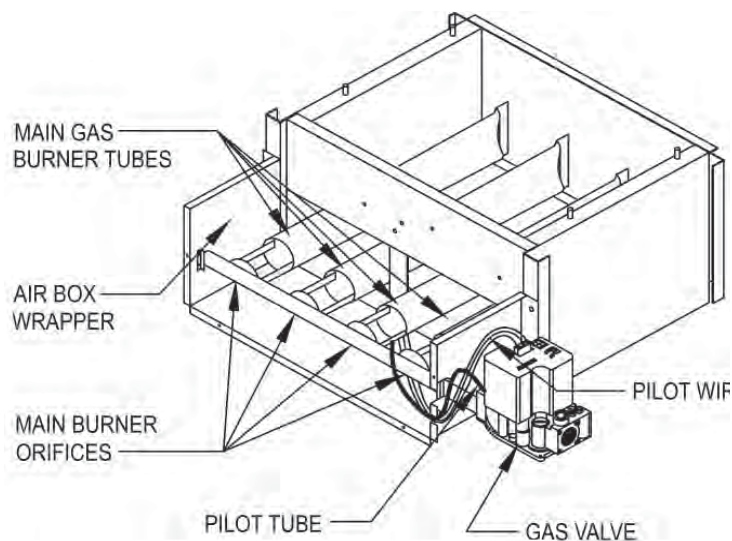
Figure 3 - Gas Burner Tubes
