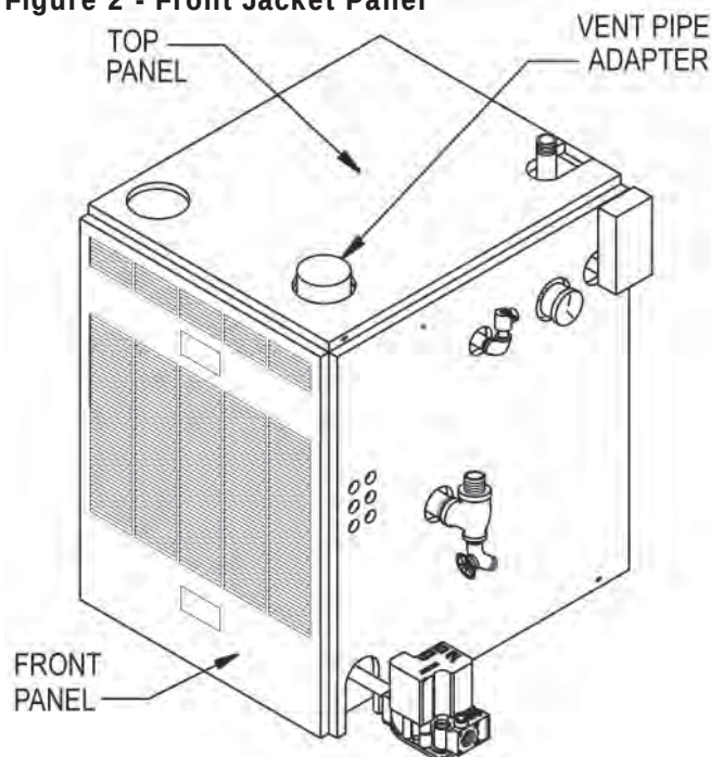
Figure 2 - Front Jacket Panel
