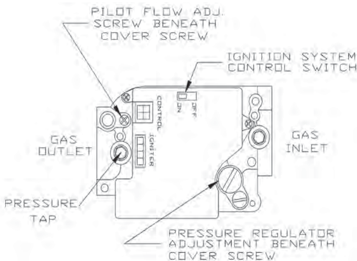
Figure 1 - Intermittent Pilot
