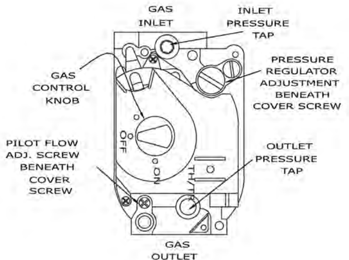
Figure 1 - Intermittent Pilot
