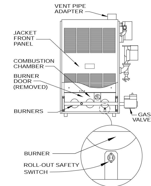
Figure 5 - Boiler Front with Safety Switch
