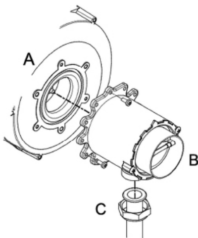
FIGURE 9-6 Venturi et buse
