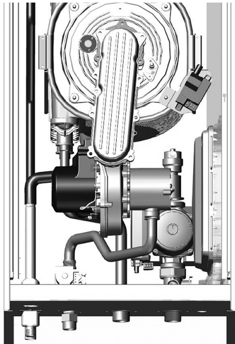
FIGURE 7-1 Raccordement au gaz
