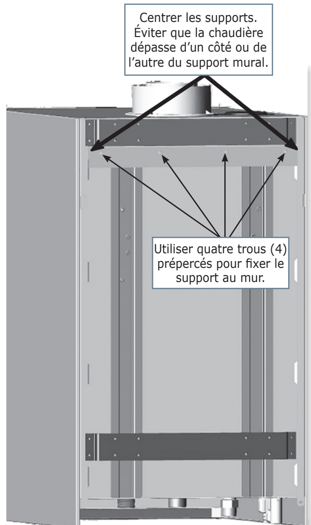
Figure 4-3 Support mural (inclus)
