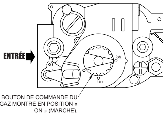
Figure 25 - Soupape de gaz
