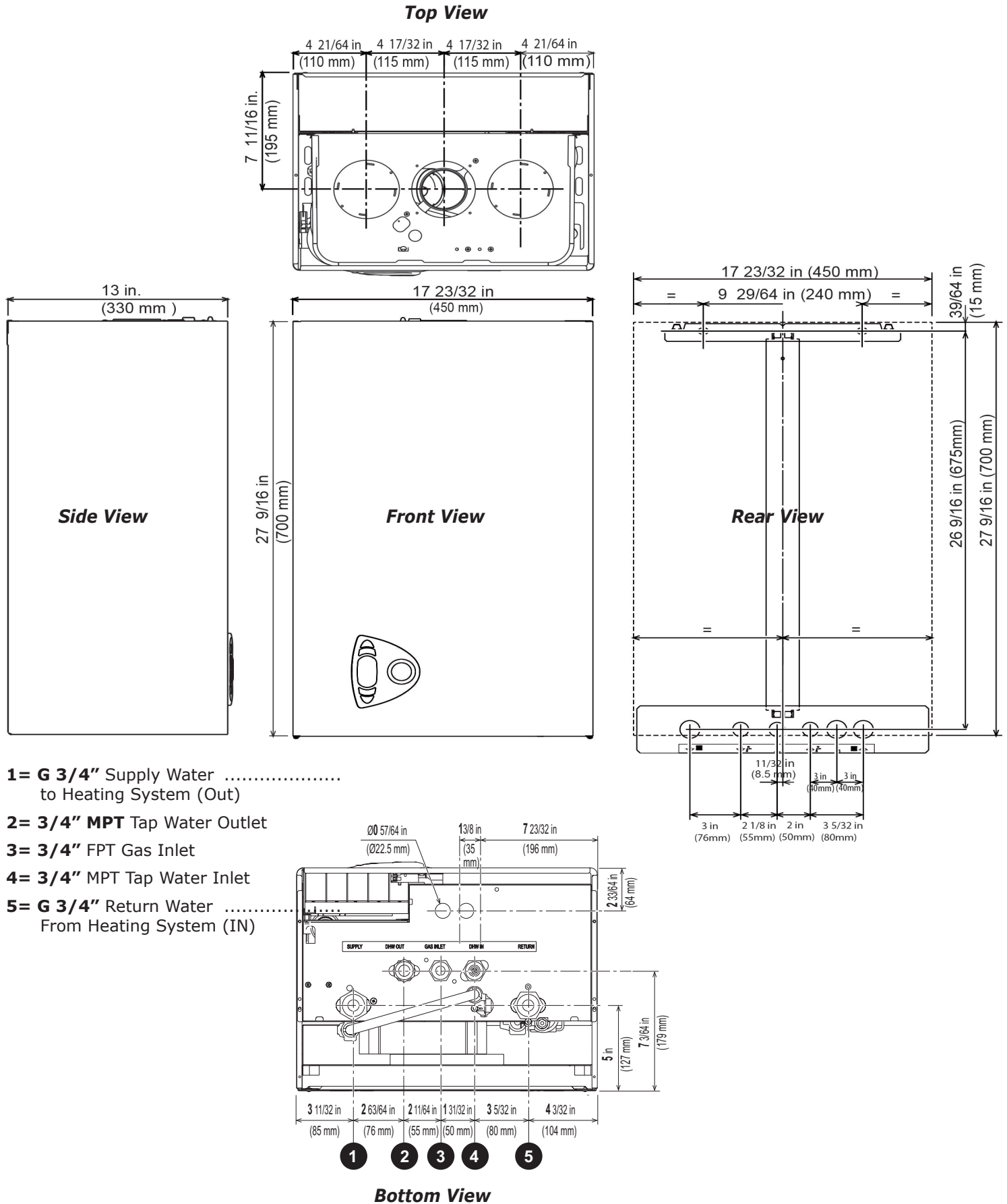
Figure 1 - Overall Dimensions
