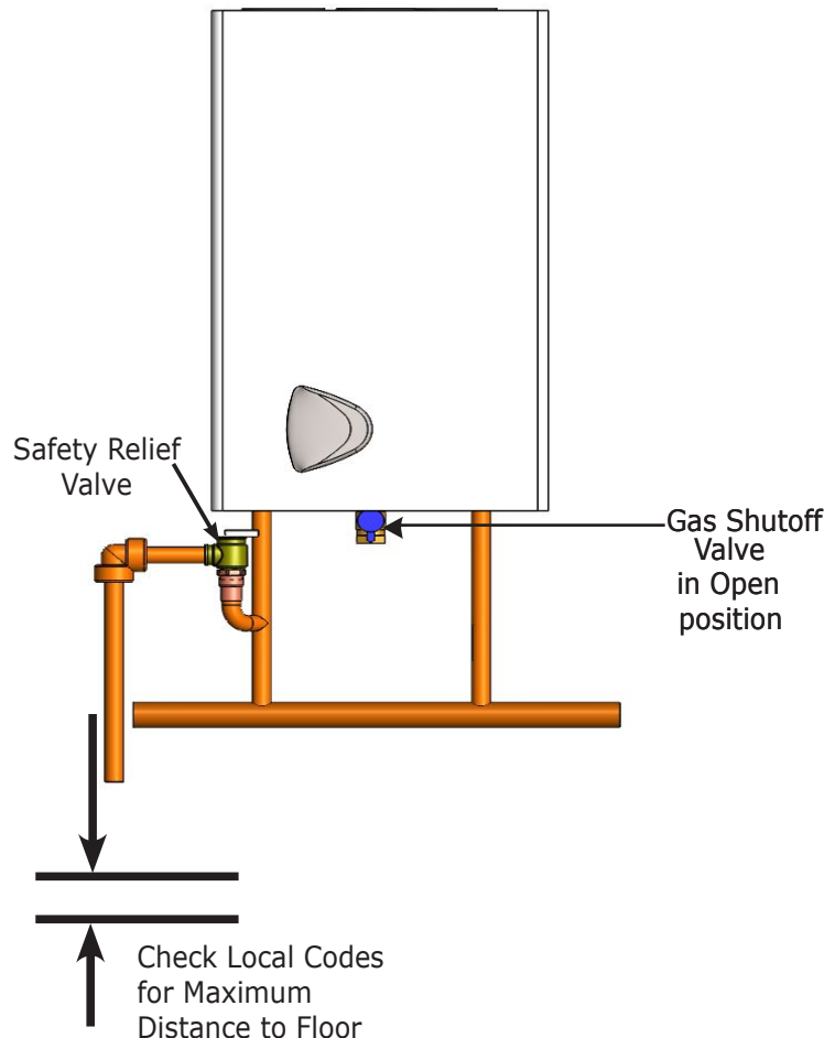
Figure 8 - Safety Relief Valve Discharge Piping
