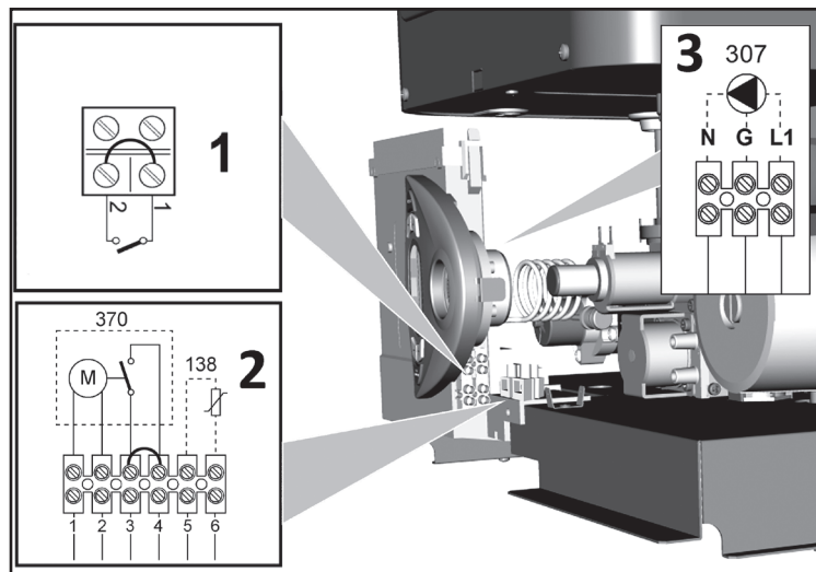
Figure 17 - Terminal Block
