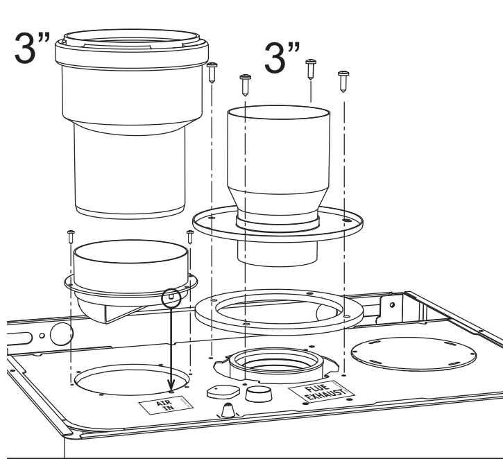
Figure 11 - Combustion Air Fitting
