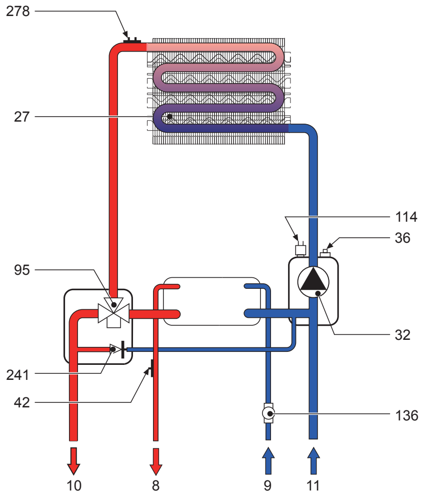
- Plumbing circuit
