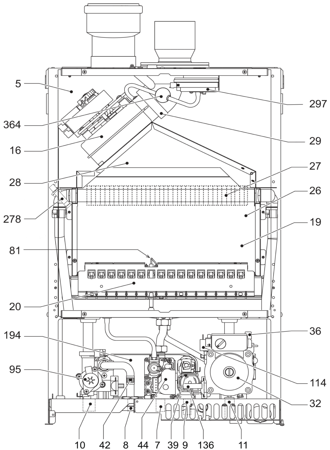
Figure 2 - Component Listing
