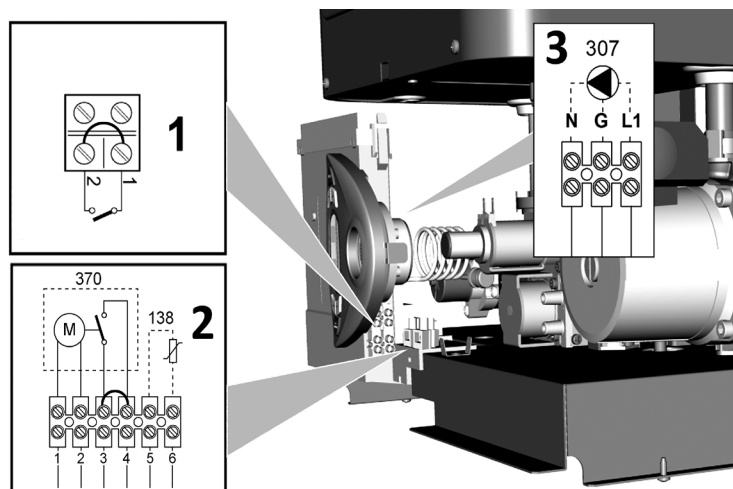
Figure 17 - Bornier
